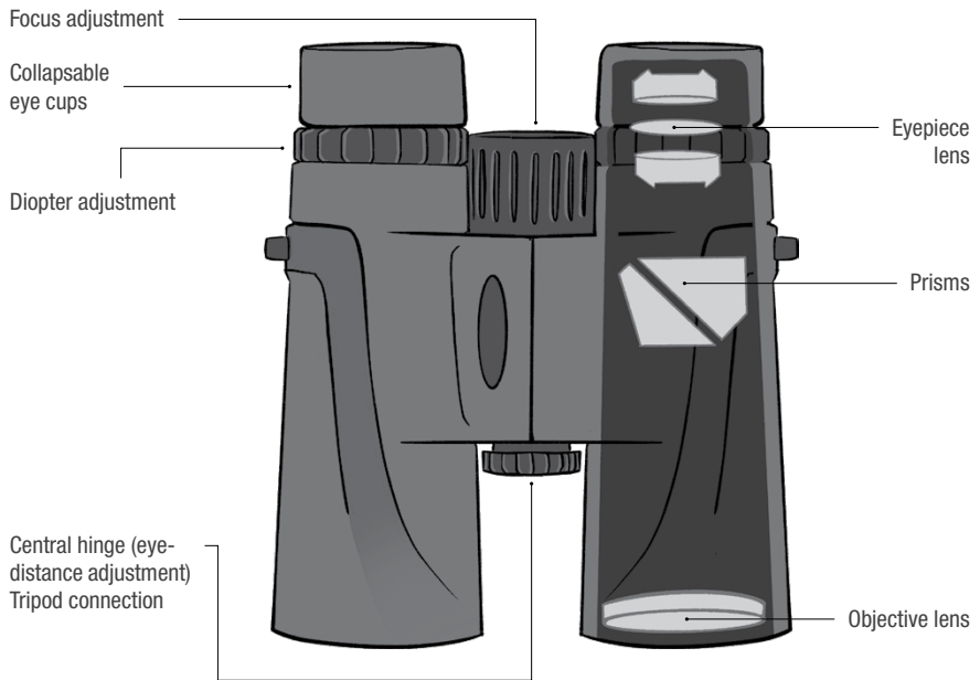
Figure 1. Names of the main parts that make up the binoculars.
