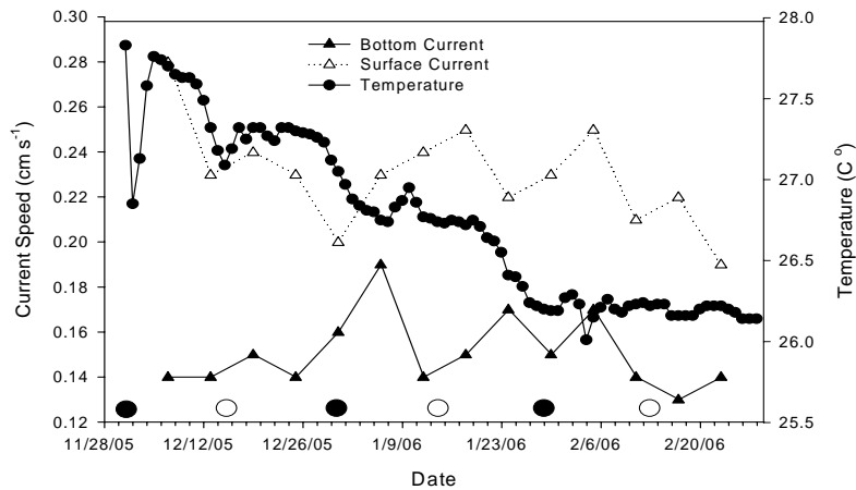
Fig 3. Temperature and surface and bottom current speed measured in relation to lunar phase on (A) Saba Bank and (B) the St. Thomas MCD from December 2005 to February 2006.
