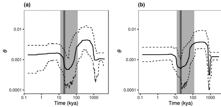
FIGURE 2 Median (solid line) and 95% confidence interval (dashed lines) of genetic diversity ( \theta ) through time (kya) estimated from the data excluding putative related individuals ( N = 44 individuals). Results are shown for (a) \mu = 7.9 \times 10^{-9} and (b) \mu = 1.2 \times 10^{-8} substitutions per site per generation. The approximate timing of the last glacial cycle (120–14 kya) is indicated in light grey shading. The LGM (26–19 kya) is indicated by a dark grey shaded bar
