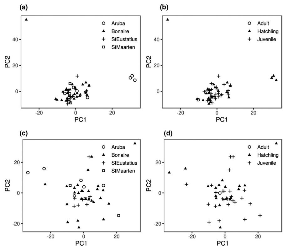
FIGURE 1 Plot of the first two principal components with individuals labelled by (a,c) sampling location (b,d) and sample type estimated from the (top panels; a–b) data including putative related individuals ( N = 53 ) and (bottom panels; c–d) data excluding putative related individuals ( N = 44 )
